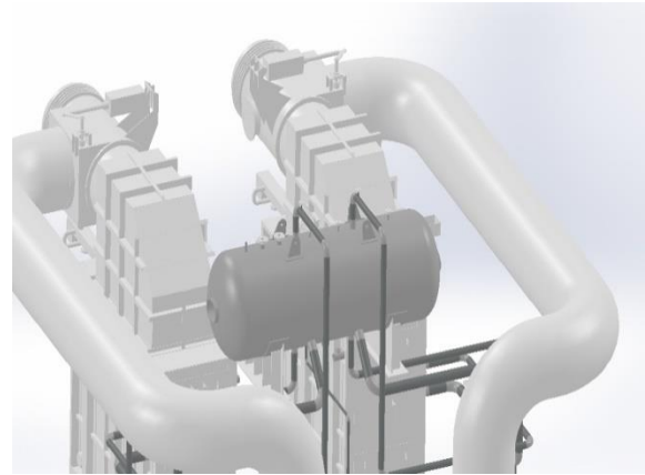
3D view of Greens Boiler
