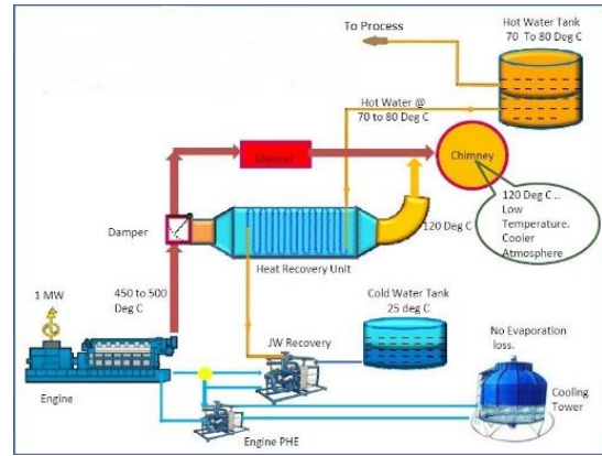
Waste Heat Recovery Hot Water system at Square Hospitals Ltd.
