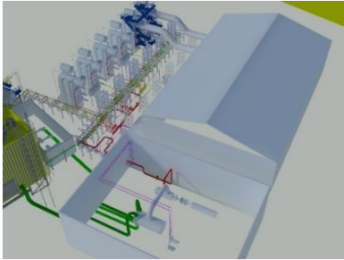
Karnaphully Power Limited 110 MW HFO (Co Generation BOP-Design, Drawing, Erection, Supply )
